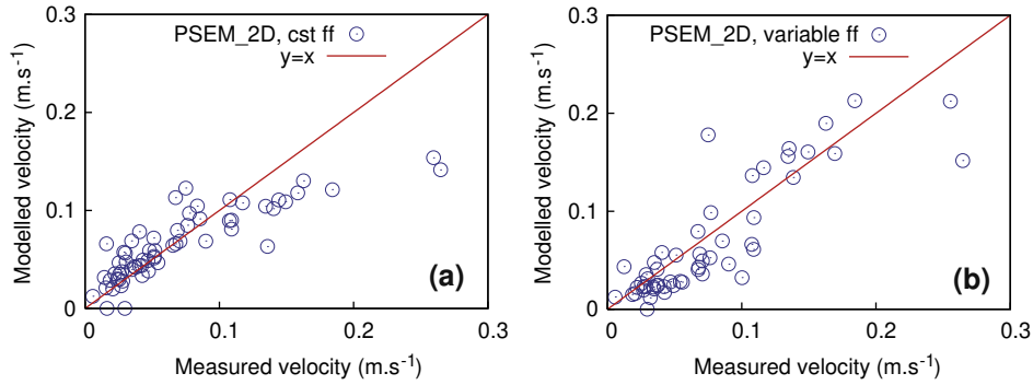
Fig. 3. Modelled versus measured velocities obtained from PSEM_2D with: (a) a constant friction factor f , (b) a varying friction factor f (see Figs. 4 and 5 in (Tatar et al., 2008)).
