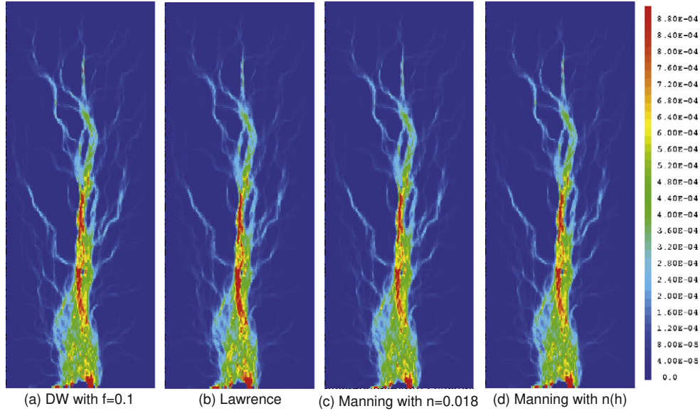
Fig. 9. Flux hu ( \text{m}^2 \text{s}^{-1} ) calculated with (a) Darcy-Weisbach's model with f constant equal to 0.1; (b) Lawrence's model with P = 13\% and h_c = 0.5 mm. (c) Manning's model with n constant equal to 0.018; (d) Manning's model with n(h) given by Eq. (6) with n_0 = 0.018 , h_0 = 3 mm and \varepsilon = 1/3 .
