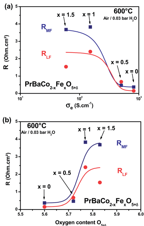
Fig. 9 Variation of the Middle Frequency (MF) and Low Frequency (LF) resistances of \text{PrBaCo}_{2-x}\text{Fe}_x\text{O}_{5+\delta} electrodes ( x = 0, 0.5, 1 and 1.5 ), at 600 \text{ }^\circ\text{C} under moist air ( 0.03 \text{ bar H}_2\text{O} ) as a function of: (a) the electrical conductivity and (b) the oxygen content (data from Fig. 3 and 4) (lines are guides for the eyes).
