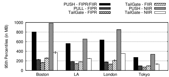
Fig. 4. 95th percentile bandwidth, for all contents.
