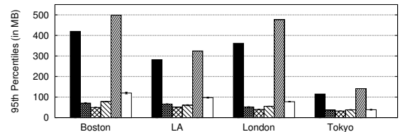
Fig. 5. 95th percentile bandwidth, for LT contents.
