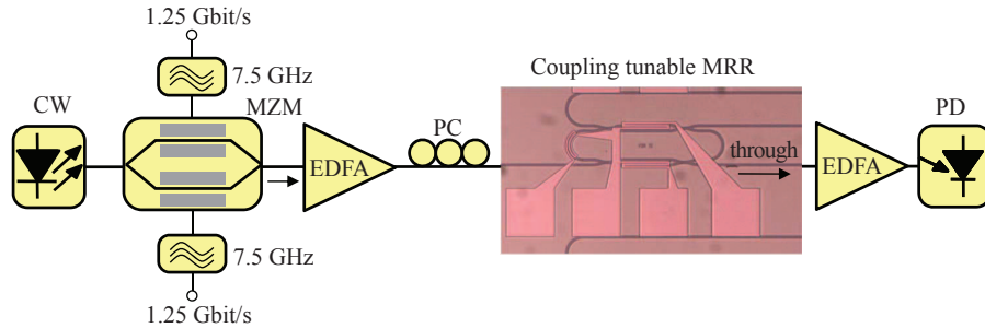
Fig. 5. Experimental setup.
