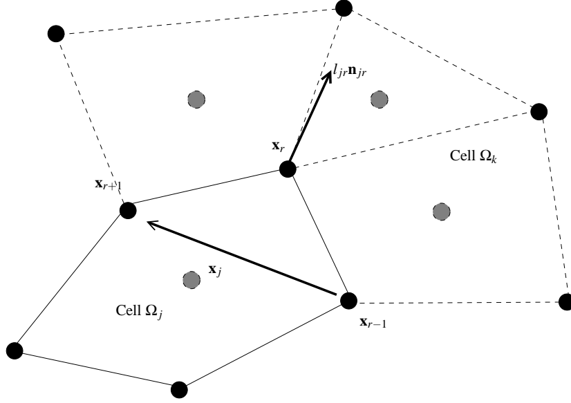
Figure 4: Notation for node formulation. The corner length l_{jr} and the corner normal \mathbf{n}_{jr} are defined in equation (20). The point \mathbf{x}_j is an arbitrary point inside the cell, typically the centroid of the cell or an averaged of the corners.
