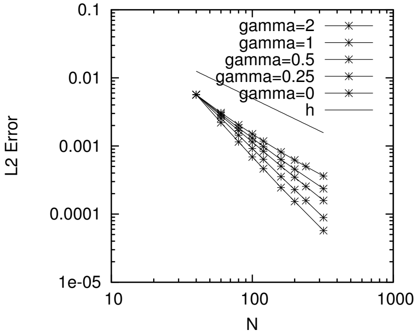
Figure 6: The error is plotted in log scale versus the number of cells per direction in the academic square. Each curve corresponds to a value of \gamma \in \{0, \frac{1}{4}, \frac{1}{2}, 1, 2\} , plus a reference line for order one. One sees that the order of convergence is an increasing function of \gamma .
