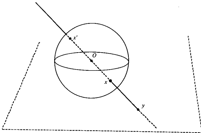
Fig. 1. The projective plane.
