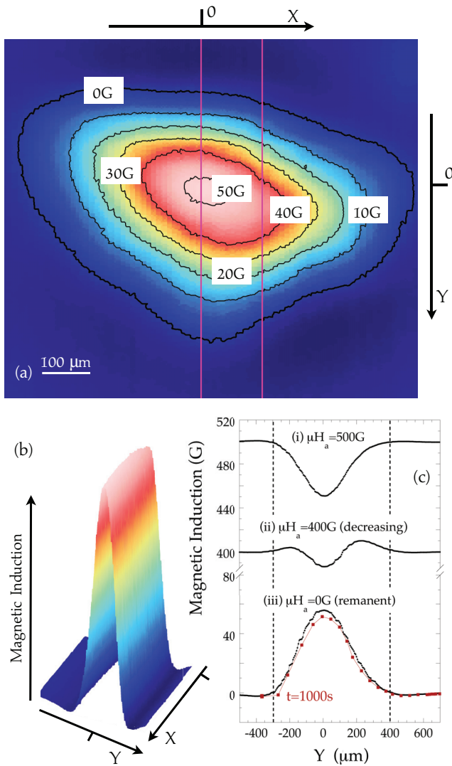
FIG. 1. (Color online) (a) Contour plot of the magnetic induction perpendicular to the sample surface obtained after cycling the field up to 500 G ( H_a \parallel c ) and back to zero (sample A). As shown in (b) the field profile in the purple rectangle clearly displays a sand-hill shape characteristic of bulk pinning. Correspondingly a V-shape profile is obtained for increasing field [see curve (i) at 500 G in (c)] and the profile is progressively reversed as the field is decreased [see curve (ii) and (iii) for H_a = 400 G and 0 G, respectively]. The solid (red) symbols for H_a = 0 have been recorded after a 1000 s waiting time, clearly showing the decay of the trapped sand hill with time (sample edges are indicated by vertical dotted lines).
