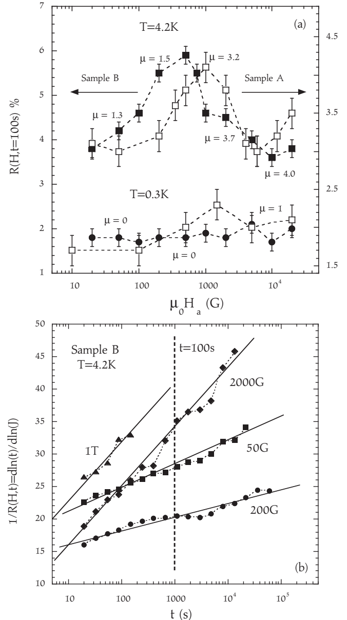
FIG. 4. (a) Magnetic field dependence of the logarithmic relaxation rate R = d \ln(J)/d \ln(t) at t = 100 s for the indicated T values in sample A (open squares, right scale) and sample B (solid symbols, left scale). Relaxation exponent ( \mu ) values are indicated for some characteristic fields, note that \mu rapidly increases above the R(H) peak. The dotted lines are guides to the eyes. (b) 1/R as a function of t (Sample B, T = 4.2 K) for the indicated H_a values. As shown the slope of the curve ( \mu ) increases at high fields (see text for details).
