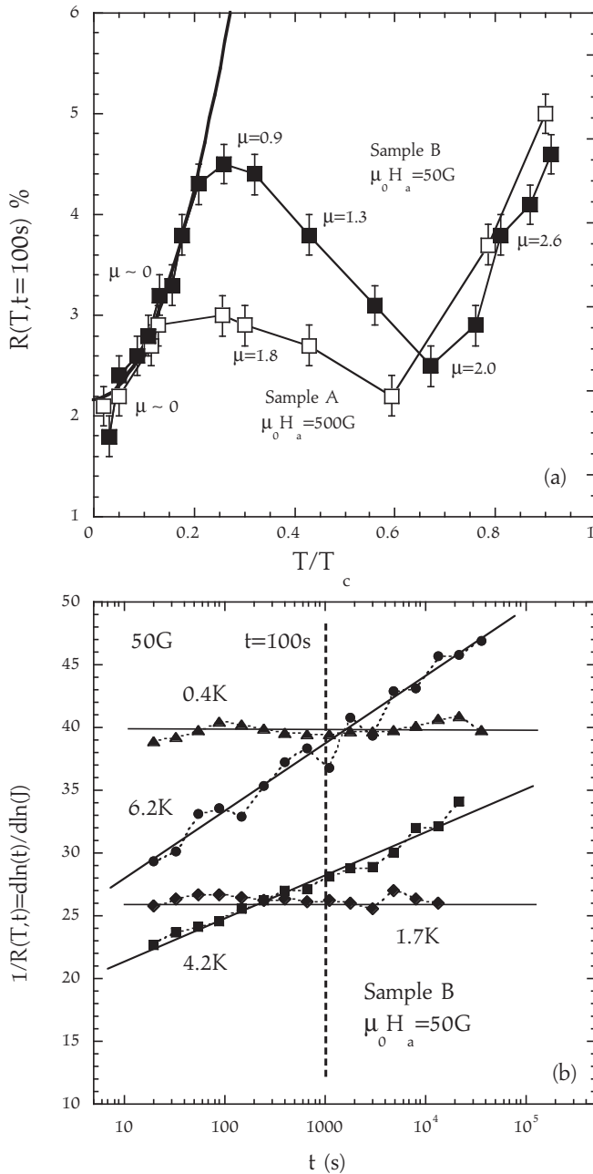
FIG. 3. (a) Temperature dependence of the logarithmic relaxation rate R = -d \ln(J)/d \ln(t) at t = 100 s for the indicated field values in sample A ( T_c \sim 14 K, open squares) and sample B ( T_c \sim 10 K, solid squares). Thin lines are guides to the eyes and the thick solid line is a R(0) \times [1 + (T/T_0)^2] fit to the data (see text for details). Relaxation exponent ( \mu ) values are indicated for some characteristic temperatures, note that \mu rapidly increases above the R(T) peak. (b) 1/R as a function of t (Sample B, \mu_0 H_a = 50 G) for the indicated T values. As shown the slope of the curve (i.e. \mu ) is close to 0 below \sim 2 K and increases at higher temperatures (see text for details).
