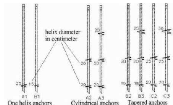
Figure 6. Prototype helical anchors tested at the CRHEA site.
