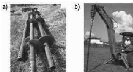
Figure 1. a) Helical anchors; b) Anchor installation.
