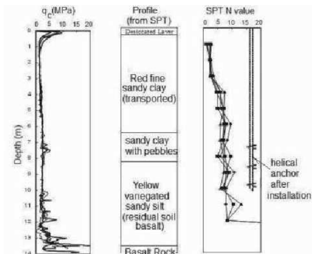
Figure 7. Soil profile at the CRHEA site.
