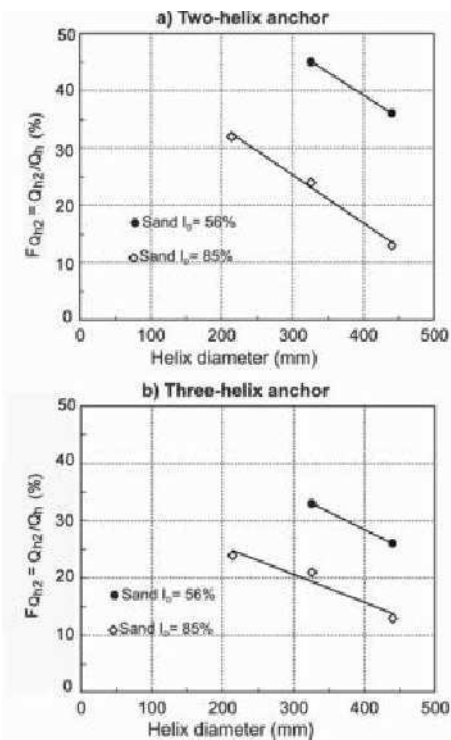
Figure 4. Relationship between the second helix contribution to total helix bearing capacity and the helix diameter of a) double helix and b) triple-helix anchors (Tsuha et al. 2012).
