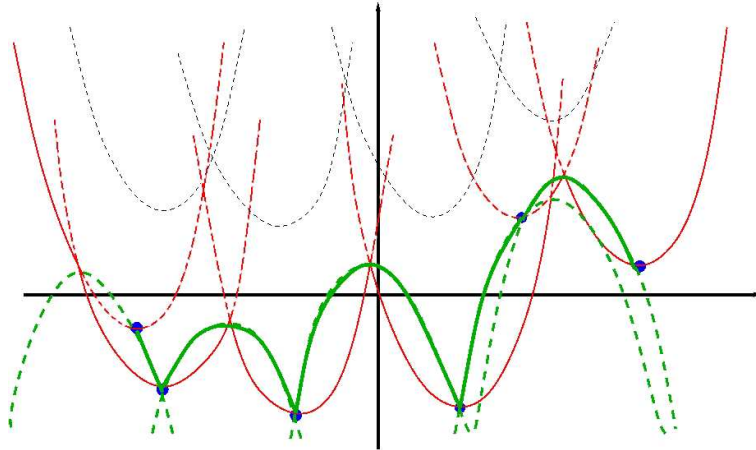
Figure 1: The point process \text{Ext}(\mathcal{P}) (blue); the boundary of the germ grain model \partial(\Phi(\mathcal{P})) (red); the Burgers' festoon \partial(\Psi(\mathcal{P})) (green).
