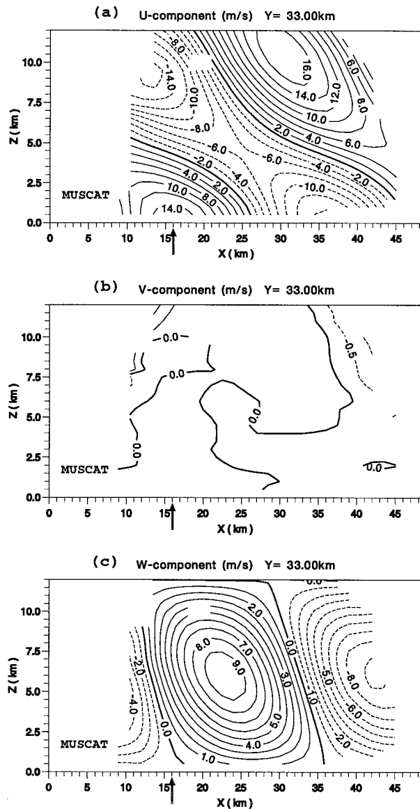
FIG. 9. Contours of (a) u , (b) v , and (c) w in the vertical plane at y = 33 \text{ km} , as obtained from MUSCAT. Aircraft position is identified by the vertical arrow below the horizontal axis.
