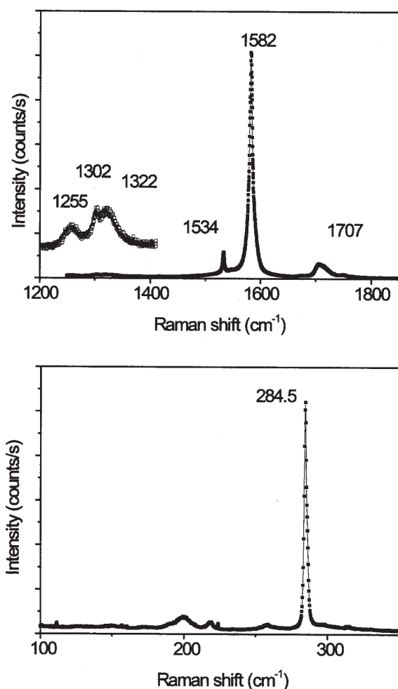
Figure 5. Raman spectra (488 nm) of radial and tangential mode energy range. One radial breathing mode is observed ( 284.5 \text{ cm}^{-1} ) which corresponds to a tube diameter 0.8 nm. The corresponding D mode is absent and the G mode is down-shifted.
