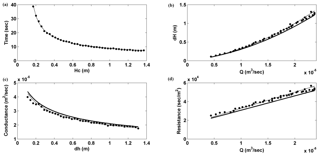
Fig. 5. Experimental results obtained for 1–2 configuration ports. (a) Control head H_c versus time. (b) Average flow rate Q versus difference head evaluated as dh = H_c + (h_0 + h_1)/2 . (c) Difference head versus conductance term evaluated as Eq. (13). (d) Average flow rate versus resistance term evaluated as the inverse of conductance. Dots represent the experimental values, dashed line represent the fitting of experimental values, and marked line represent the functions without the effect of circuit ( C = 0 ).
