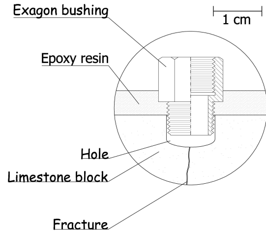
Fig. 3. Illustration of a “port” construction details.
