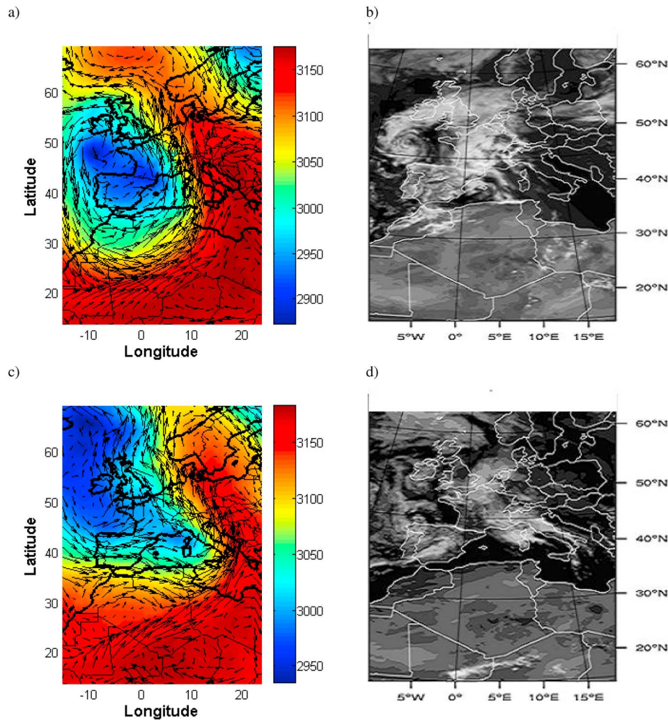
Figure 1. Synoptic situation on (top) 27 May and (bottom) 29 May 2008: (a and c) 700-hPa geopotential height (shading) and wind (vectors) at 1200 UTC from ECMWF analyses and (b and d) Meteosat Second Generation (MSG) images at 0.6 \mu\text{m} (at 1200 UTC 27 May (Figure 1b) and 1230 UTC 29 May (Figure 1d)).
