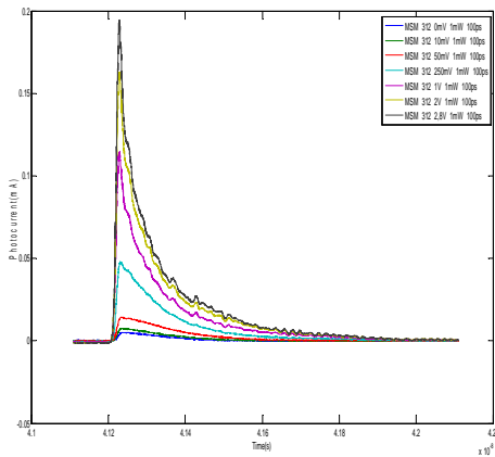
Fig. 3. Pulse response of GaAs MSM312 photoswitch at \lambda=780\text{nm} with different bias voltages ( P_{opt}=1\text{mW} , A=3 \times 3 \mu\text{m}^2 , s=l=1 \mu\text{m} )
