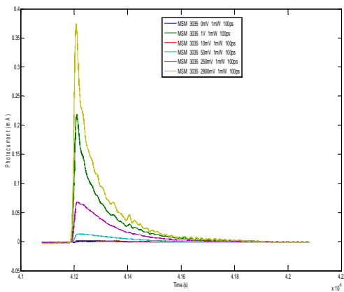
Fig. 4. Pulse response of GaAs MSM3035 photoswitch at \lambda=780\text{nm} with different bias voltages ( P_{opt}=1\text{mW} , A=3 \times 3 \mu\text{m}^2 , s=l=1 \mu\text{m} )
