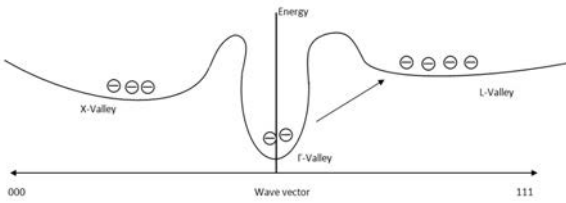
Fig. 6. Gunn Effect
