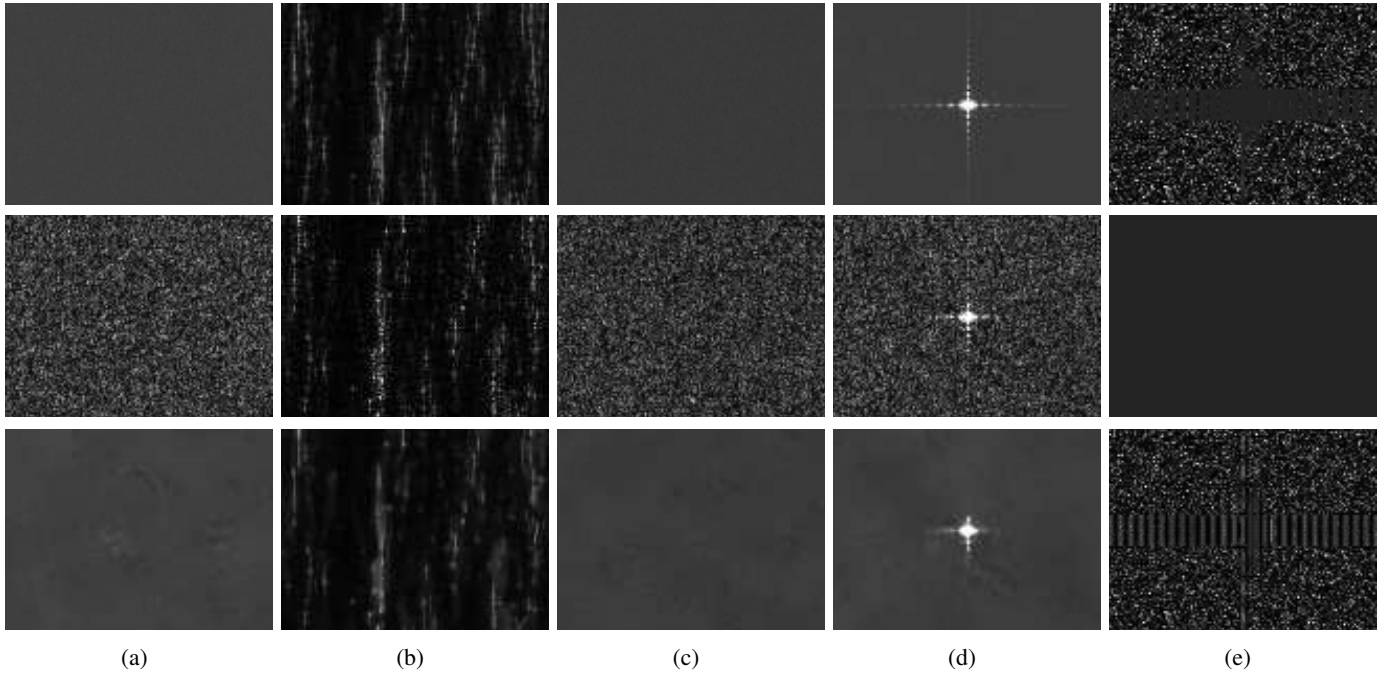
Fig. 6. Restoration with NL-SAR of 5 test cases proposed in [Di Martino et al., 2013]: (a) homogeneous region; (b) texture (image of a synthetic fractal DEM); (c) squares image; (d) point target; (e) building.
