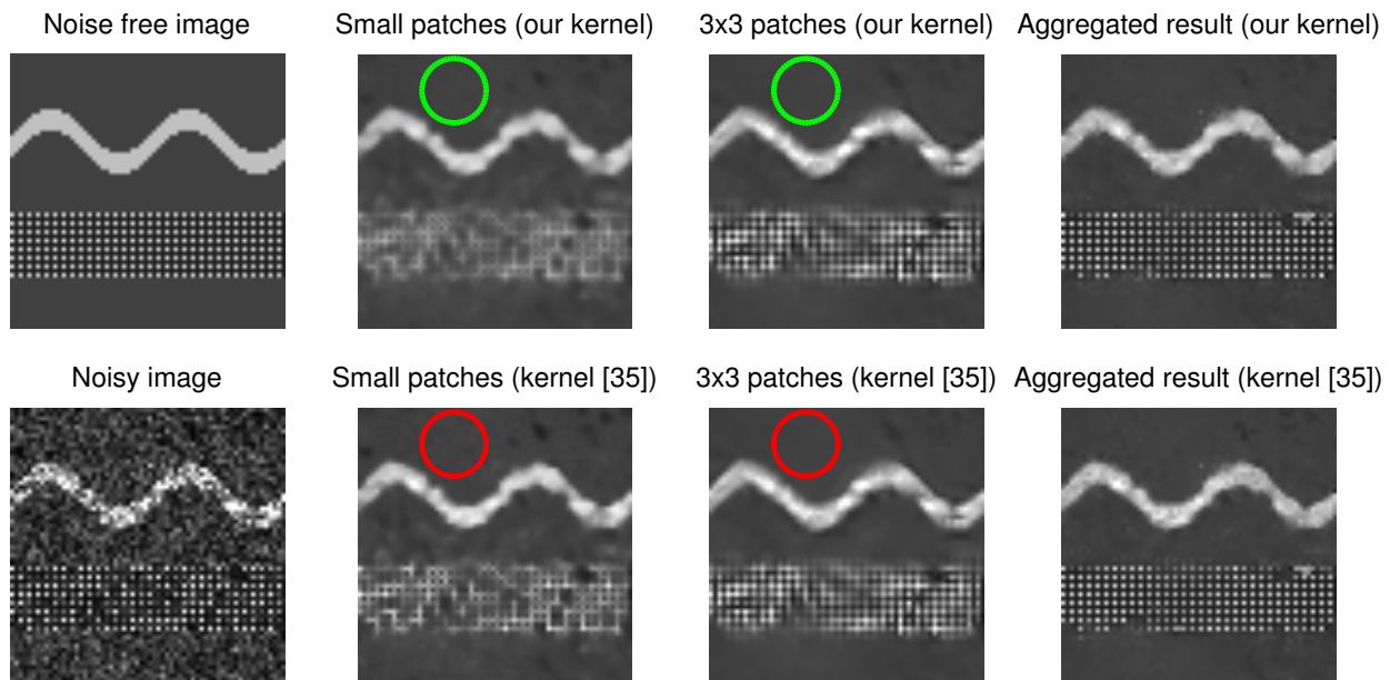
Fig. 3. Comparisons between kernels that adapt to the distribution of the criterion versus kernel based on moments of the criterion only (similar to the one of [Kervrann and Boulanger, 2008]). Green circles illustrates that the first kernels ensure a same level of noise reduction in homogeneous regions, while red kernels illustrates that the second kernel does not.
