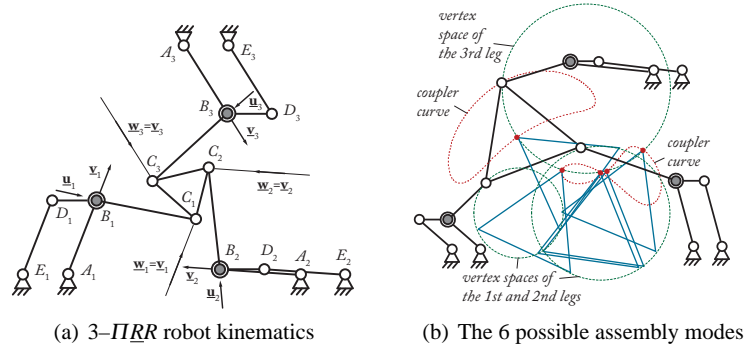
Fig. 3 The hidden robot model of the 3- \underline{RRR} robot and its hidden robot model
