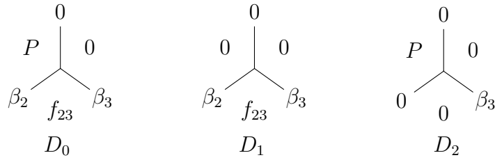
Figure 7: Y-diagrams
