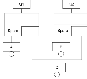
Figure 7: Two Spare gates sharing a spare event
