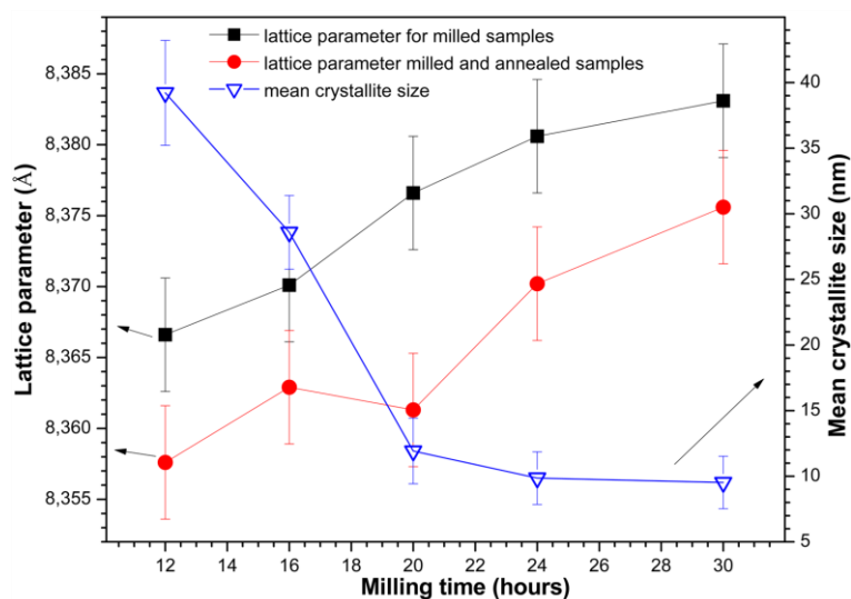
Fig. 2. Evolution of the mean crystallite size and of the lattice parameter of the \text{NiFe}_2\text{O}_4 for as-milled samples and respectively for milled and annealed samples versus milling time.
