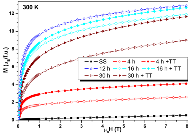
Fig. 4. Room temperature magnetization curves of the starting sample, milled for 4, 12, 16 and 30 hours samples and milled and subsequently annealed (350 °C/4 hours) samples.
