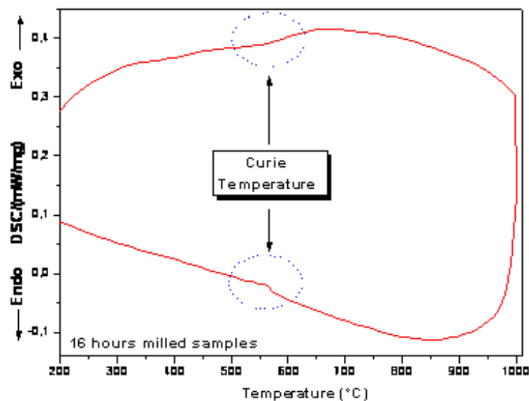
Fig 3. DSC heating and cooling curves for the sample milled 16 hours. The peaks corresponding to the magnetic transition of the \text{NiFe}_2\text{O}_4 on the heating and cooling curves are marked.
