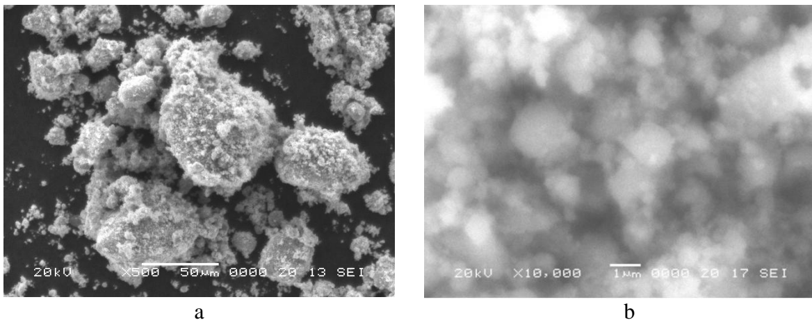
Fig. 6. SEM images of nickel ferrite powders obtained for the 16 h milled sample: a – 500x; b – 10,000x. The powder is formed by agglomeration of nanometric particles alongside by micrometric size particles.
