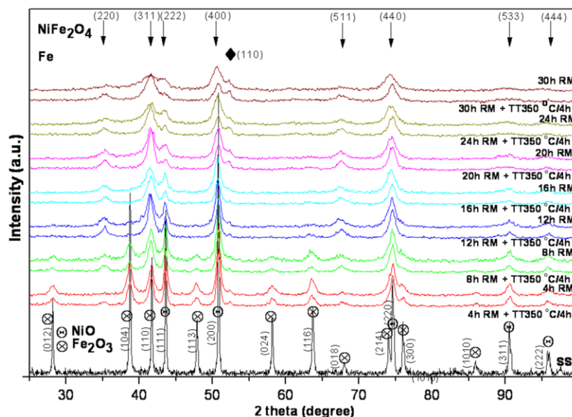
Fig. 1. X-ray diffraction patterns of the starting sample (ss), as-milled samples (4, 8, 12, 16, 20, 24 and 30 h of milling) and for the milled and subsequently annealed at 350 ^{\circ}\text{C} for 4 h samples. The position of the Bragg peak for each phase is indicated in the figure. For clarity, the diffraction patterns were vertically shifted.
