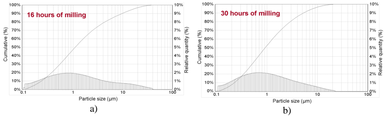
Fig. 7. Particles size distribution of \text{NiFe}_2\text{O}_4 powder milled obtained after 16 h of milling a) and respectively, 30 h of milling b).
