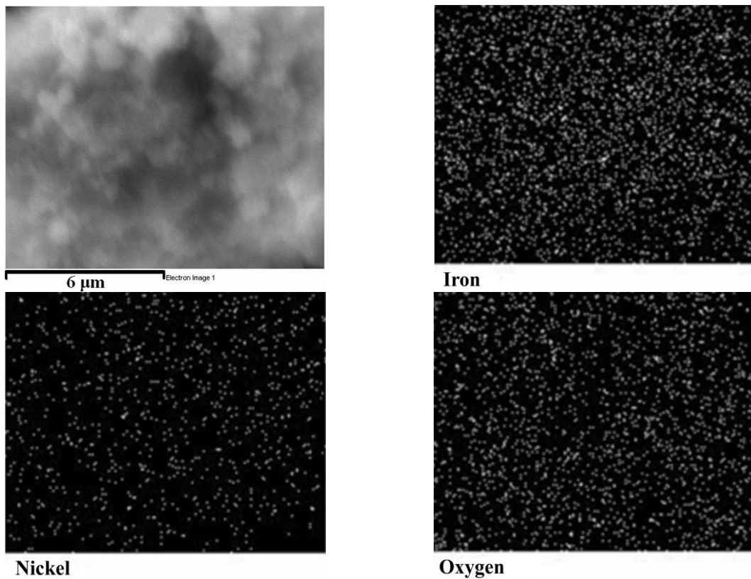
Fig. 8 Distribution maps for Ni, Fe and O chemical elements obtained for the 16 h milled sample. The X-ray microanalysis was performed on the SEM image presented in the upper left side (10,000X).
