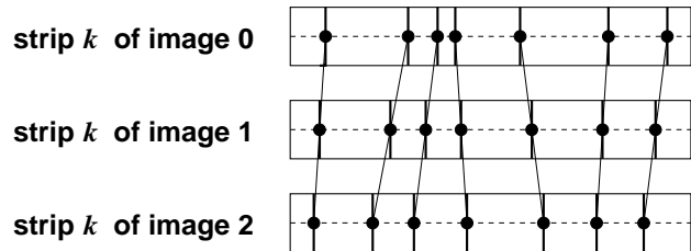
Figure 7: Multi-image strip alignment.
