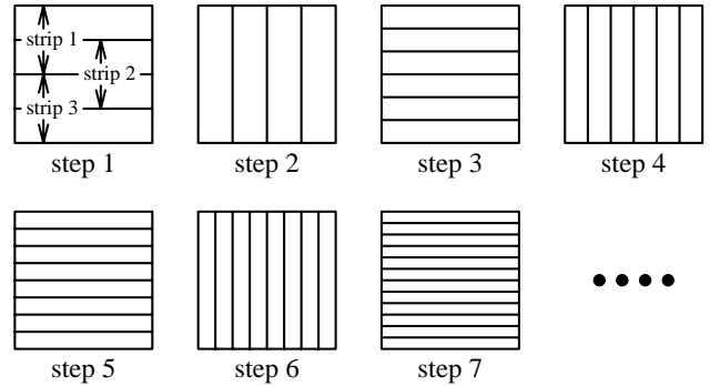
Figure 4: Strip spacing and width reduction.
