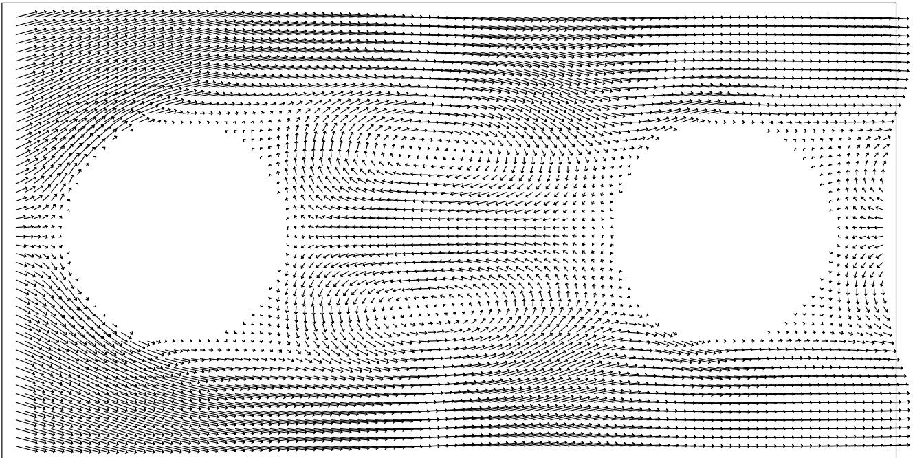
Figure 8: Synthetic particle image (top) and the “Correct” velocity field, magnified twice, (bottom). Average velocity module is 7.58 pixel/frame.
