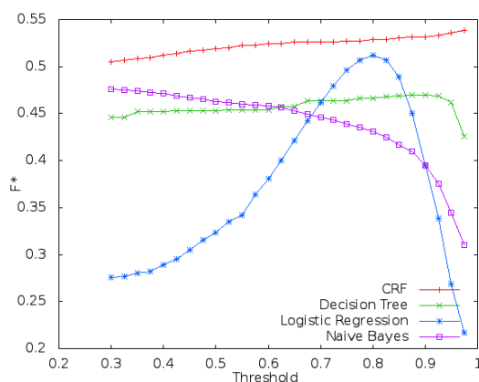
Fig. 2. Performance comparison ( F^* ) among different classifiers
