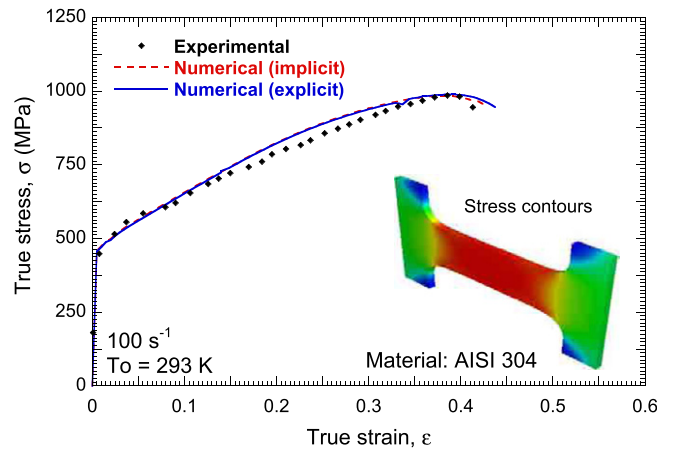
Fig. 10. Stress-strain curve in dynamic tensile test at \theta_0 = 293 K and \dot{\epsilon} = 100 s^{-1} . Comparison between experimental results (Rodríguez-Martínez et al., 2011a) and numerical results using implicit (Zaera et al., 2012) or explicit schemes for the integration of the constitutive model.
