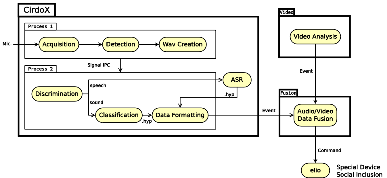
Fig. 1. Organisation of CirdoX and its insertion into the global system.
