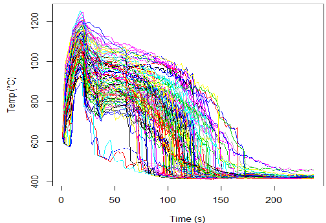
Figure 1: Visualization of the BEMUSE data: 100 temporal curves of the cladding temperature of the fuel rods. Each curve comes from the output of one computer code (CATHARE2) run. Source: CEA.
