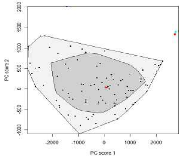
Figure 6: Bagplot of BEMUSE study case.
