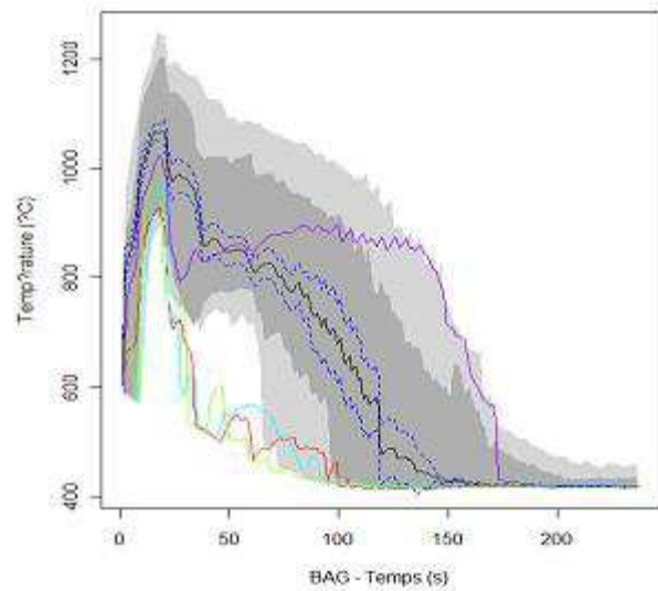
Figure 7: Bagplot results in the functional space for BEMUSE study-case.
