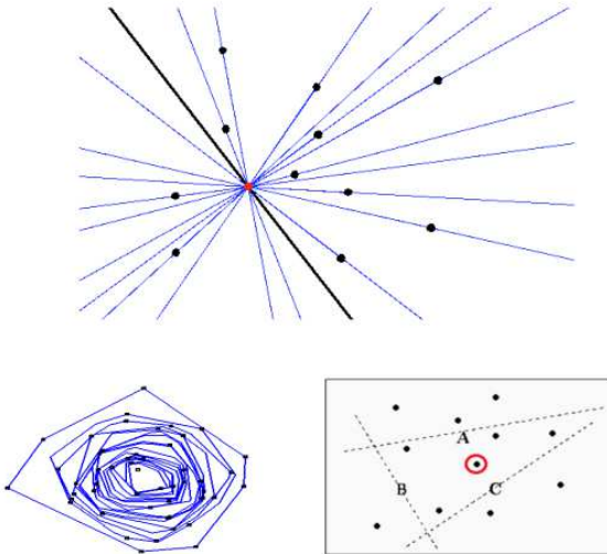
Figure 5: Illustration of the depth of Tukey.
