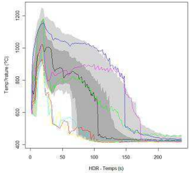
Figure 4: BEMUSE study-case: Visualization of functional quantiles and outliers, back in the physical space.
