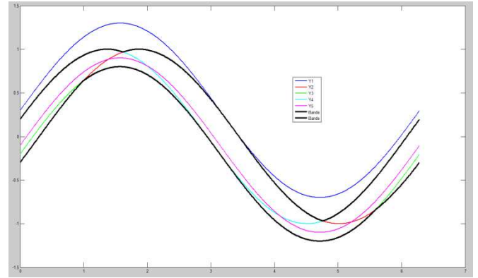
Figure 9: Example of band of curves.
