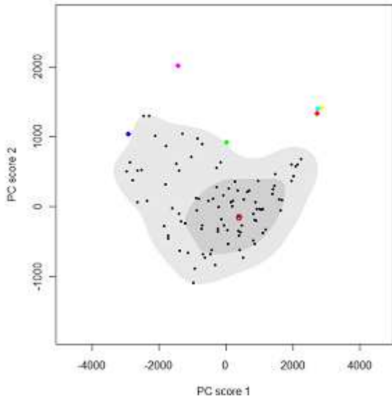
Figure 2: Visualization of the density estimator on the BEMUSE study case. Dark grey zone envelops 50% of the distribution. Light grey represents 95% quantile zone.
