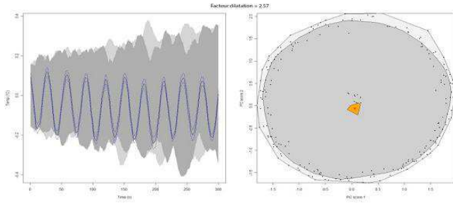
Figure 8: Example of a non-unimodal problem, where bagplot is not relevant.
