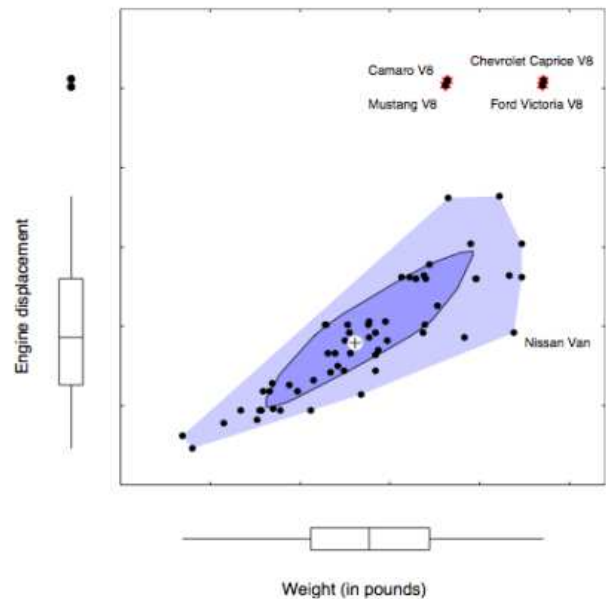
Figure 4: Example of bagplot (Source: Rousseeuw et al. 8) ).
