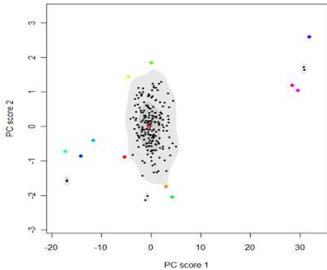
Figure 3: Visualization of a density estimator on another example. Some outliers being very close from each other: high density regions may be wrong in this case.
