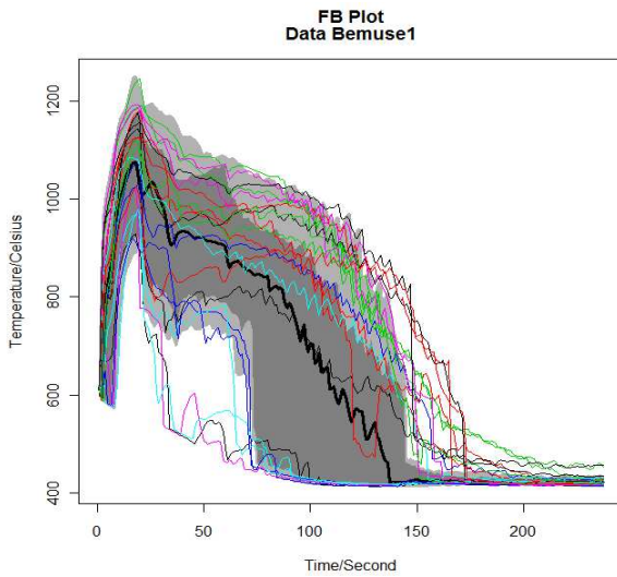
Figure 11: Functionnal boxplot of BEMUSE study-case.
