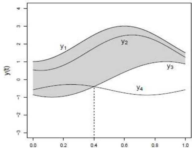
Figure 10: Illustration of band depth. Source: Sun and Genton 7) .
