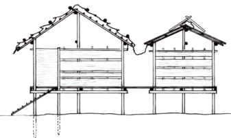
Ringle house (Malaysia) Heavy rains, floods
