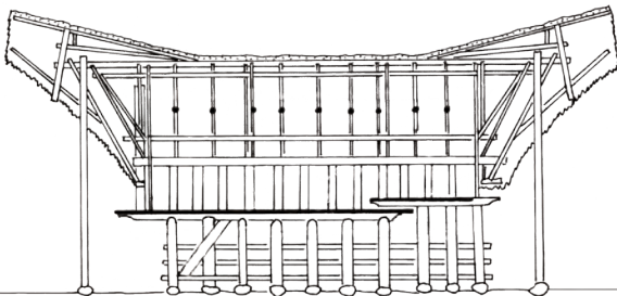
Guantanan Toraja house (Indonesia) Heavy rains, strong winds
