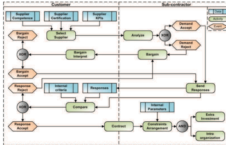
Fig. 2. Long term coordination process model
