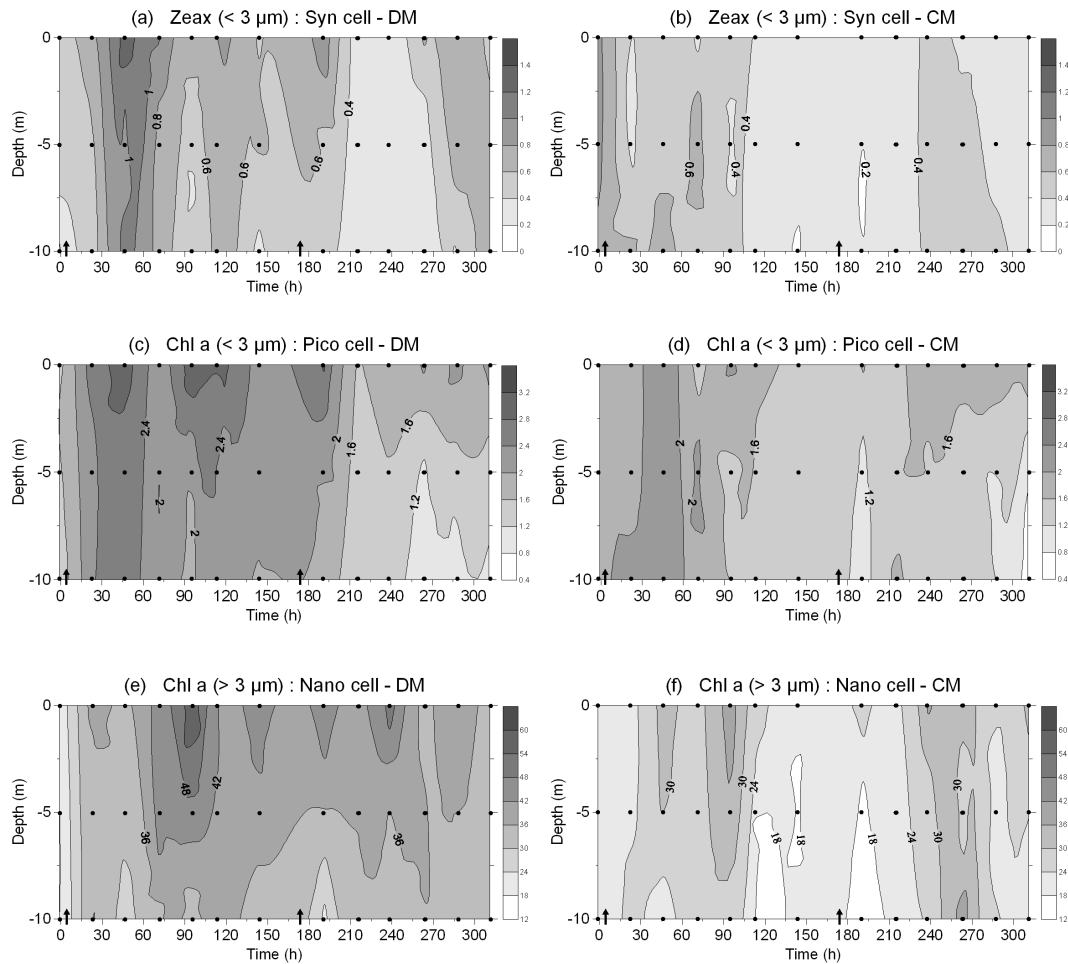
Fig. 5. Evolution of picophytoplankton mean zeaxanthin ( Zeax_{<3>} ) concentration per Synechococcus cell ( fg\ Zeax_{<3>}\ cell^{-1} ) in dust-amended mesocosms (DM; (a) ) and control mesocosms (CM; (b) ), picophytoplankton mean chlorophyll (Chl) a_{<3>} concentration per the sum of Synechococcus and picoeukaryotes cell ( fg\ Chl\ a_{<3>}\ cell^{-1} ) in DM (c) and CM (d) , and nanophytoplankton mean Chl a_{>3} concentration per cell ( fg\ Chl\ a_{>3}\ cell^{-1} ) in DM (e) and CM (f) , over time (hours). Syn, Synechococcus ; Pico, picophytoplankton; Nano, nanophytoplankton. The arrows indicate the time at which each dust addition was performed.
