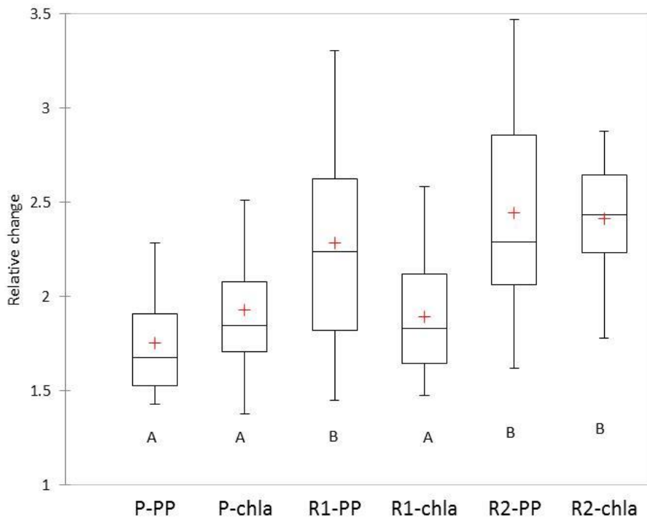
Fig. 6. Box plot of the relative changes in integrated Chl a ( \text{Chl } a_{\text{dust}}/\text{Chl } a_{\text{control}} ) and PP ( \text{PP}_{\text{dust}}/\text{PP}_{\text{control}} ) over the duration of the DUNE experiments. Means that were not significantly different between the different parameters and experiments ( p > 0.05 ) are labeled with the same letter.
