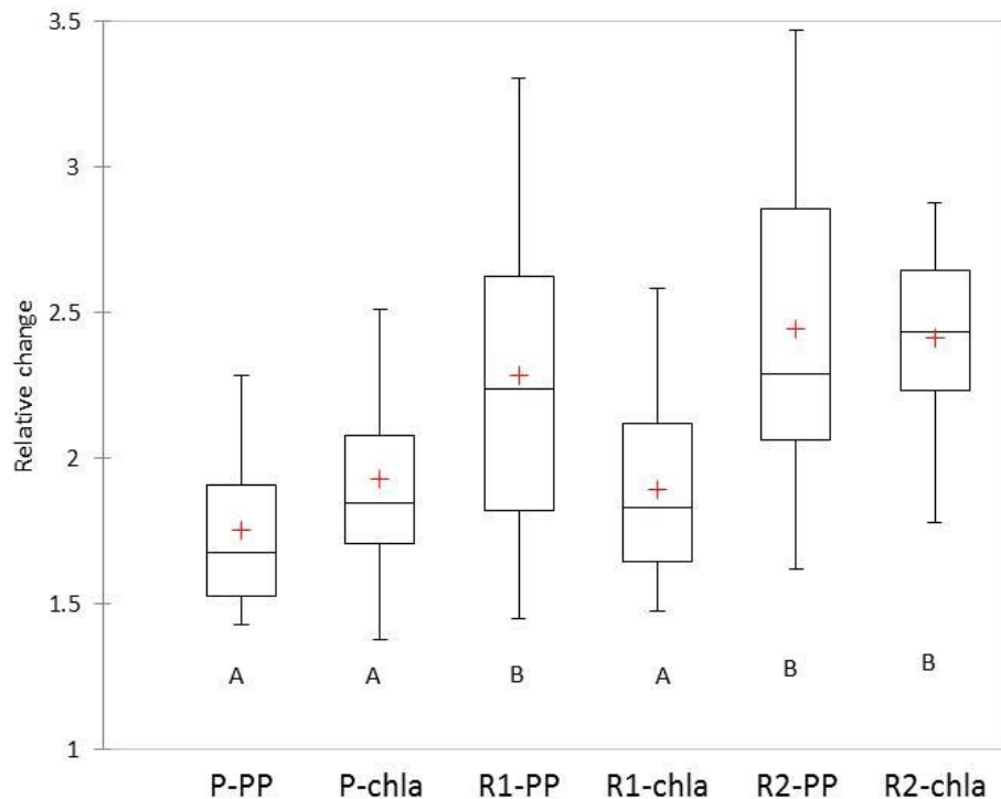
Fig. 6. Box plot of the relative changes in integrated Chl a ( \text{Chl } a_{\text{dust}}/\text{Chl } a_{\text{control}} ) and PP ( \text{PP}_{\text{dust}}/\text{PP}_{\text{control}} ) over the duration of the DUNE experiments. Means that were not significantly different between the different parameters and experiments ( p > 0.05 ) are labeled with the same letter.
