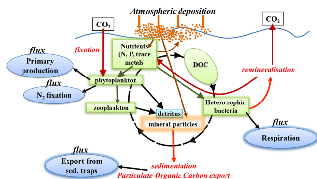
Fig. 2. Stocks (green) and fluxes (blue) measured during the DUNE experiments after the simulation of a realistic atmospheric input in a water body large enough to be representative of natural processes. As the particles are naturally sinking, those changes are closer to the “real” processes occurring in the surface mixed layer of open ocean compared to microcosm approaches where the particles are homogenized and not allowed to sink. The derived parameterizations can constrain a biogeochemical model that takes into account the atmospheric deposition in oligotrophic conditions (modified from de Leeuw et al., 2014).
