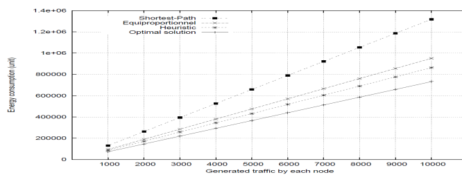
Figure 2. Maximum energy consumption (BS in the corner of a 10x10 grid)
