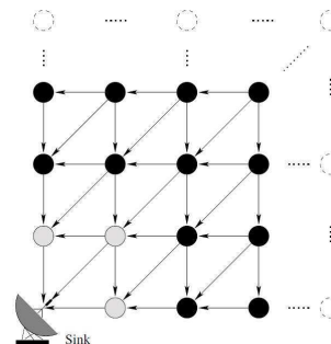
Figure 1. WSN with a grid topology and Sink in the corner. Sensors near the Sink will die faster than the other ones.
