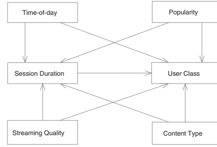
Fig. 1. User classifier
