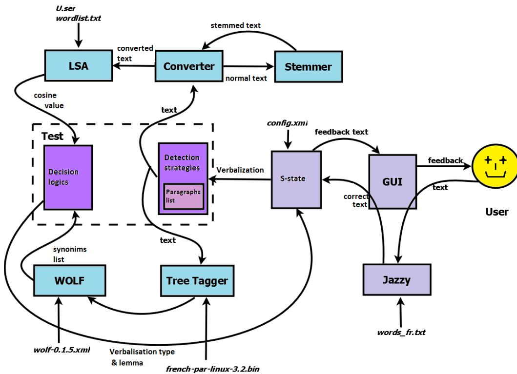
Fig. 2. Data flow
