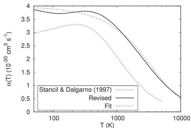
Figure 1. Rate coefficient for the process Li(2s) + H(1s) → LiH + hv.
