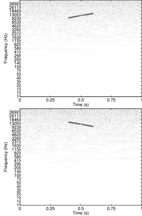
Fig. 4. Examples of CQT representation of the two localized linear chirps used in the toy dataset. These images are obtained after a 512 \times 512 resizing and a 15 \times 15 average filtering.
