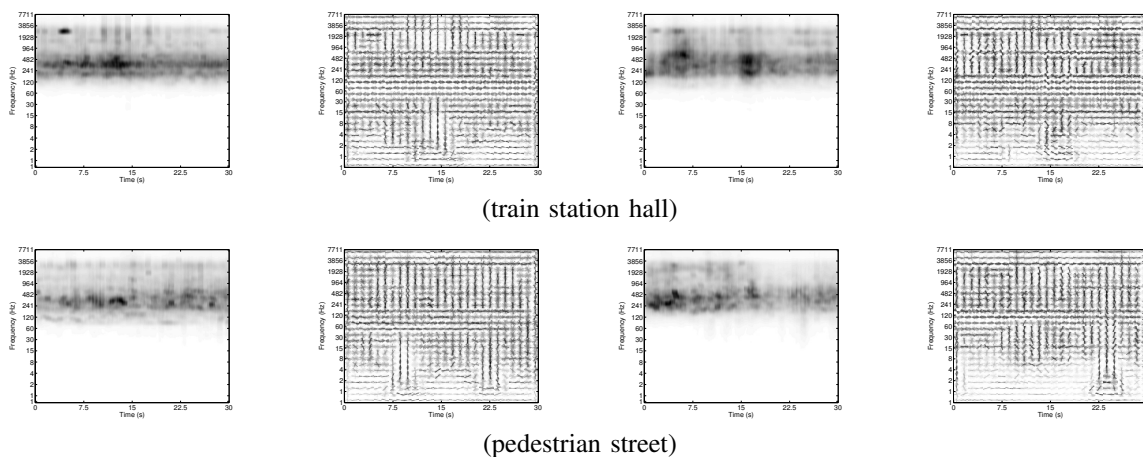
Fig. 8. Examples of CQT representation and associated HOG representations for audio scene with several people walking (top) train station hall (bottom) pedestrian street.
