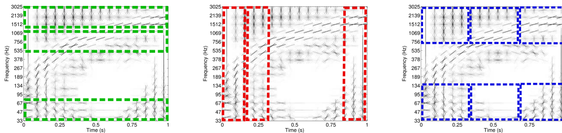
Fig. 3. Illustrating the different types of pooling we investigate based on the HOG issued from Figure 2. (Left) time pooling. (Middle) frequency pooling. (right) block-sized pooling. The green, red and blue boxes provide an example on the regions on which local histograms are averaged. The x-axis and y-axis respectively denote the time and frequency axes. Best viewed in color.
