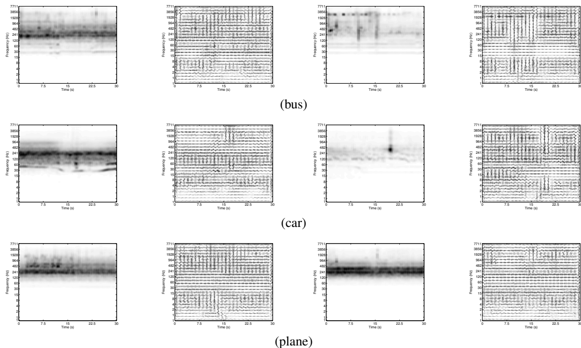
Fig. 6. Examples of CQT representation and associated HOG representations for transportation devices (top) bus. (middle) car. (bottom) plane.
