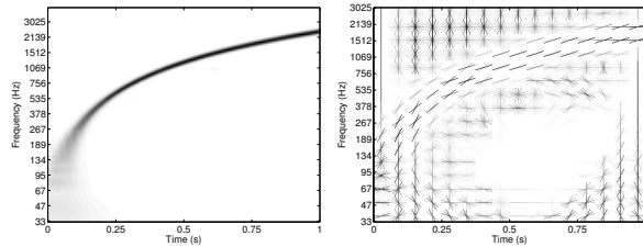
Fig. 2. Example of HOG for a toy linear chirp. (left) 512 \times 512 image of the CQ transform of the signal. (right) histogram of gradients representation of the signal. Note that for a sake of interpretation, each cell in the plots represents the occurrence of edge orientation in the cell and the darker the orientation is, the more present the orientation is. We thus note that along the chirp, the HOG representation correctly captures the direction of energy variation.
