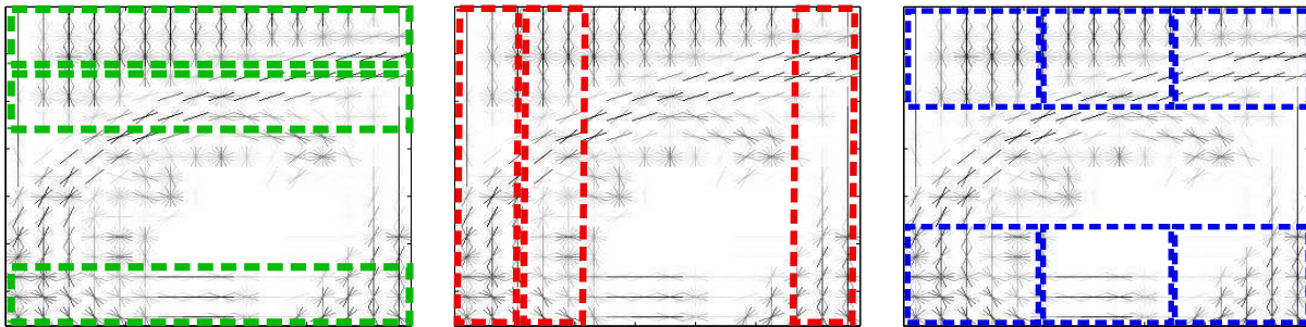
Figure 3: Illustrating the different types of pooling we investigate. (left) time pooling. (Middle) frequency pooling. (right) block-sized pooling. The green, red and blue boxes provide an example on the regions on which local histograms are averaged. The x-axis and y-axis respectively denote the time and frequency axes. Best viewed in color.
