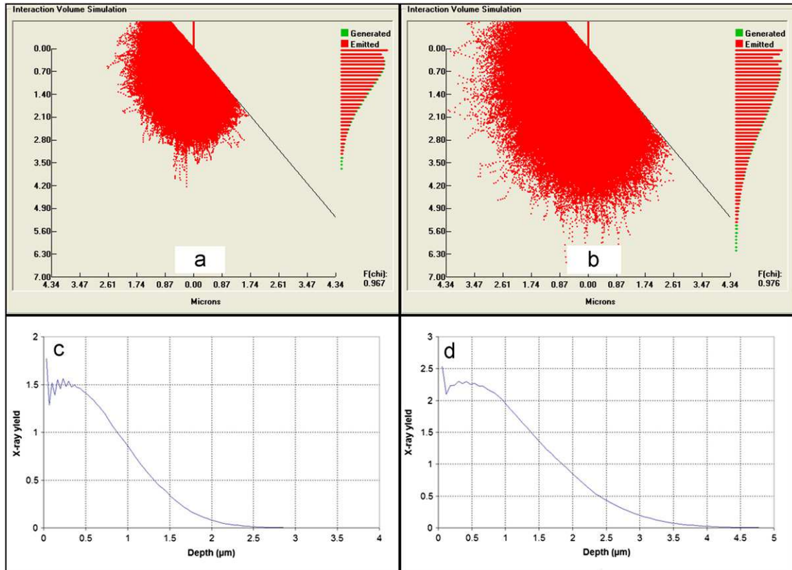
Fig. 4. Simulations of the emitted X-ray volume below the surface for copper (a) and germanium (b) and X-ray yields as a function of depth for copper (c) and germanium (d).
