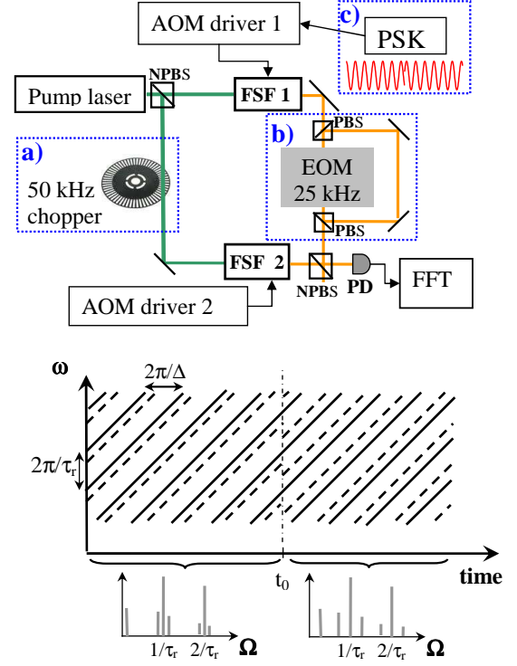
Fig. 1. Top: experimental setup showing the three different experiments -a), b) and c)- described in text. Bottom: sketch of the GMCs in the (t, \omega) representation illustrating the principle of the experiments. The GMC of laser 1 (solid) is used as a reference. At t_0 , a test parameter is changed here on laser 2: the optical light field, the path delay and the phase of the AOM driving signal in a), b) and c) respectively. A shift in the (RF) heterodyne beatings before and after the change of the test parameter indicates a shift in the GMC phase of laser 2 (dash).
