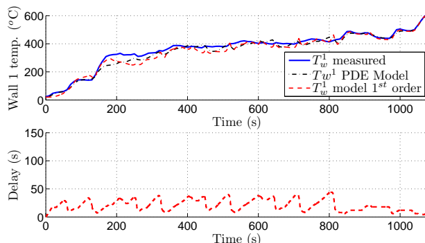
(a) Simulation results for both the proposed reduced PDE model and its approximation by an input-delay model, compared to experimental data in the center of the first monolith. Below : the corresponding delay used in the input-delay model.
