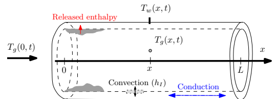
Fig. 3. Schematic view of the distributed profile temperature inside a catalyst jointly with thermal exchanges.
