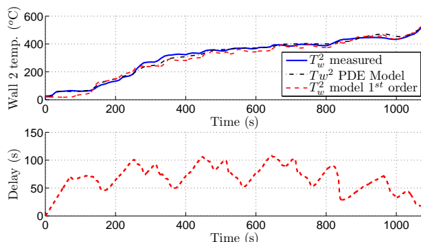
(b) Simulation results for both the proposed reduced PDE model and its approximation by an input-delay model, compared to experimental data in the center of the second monolith. Below : the corresponding delay used in the input-delay model.
