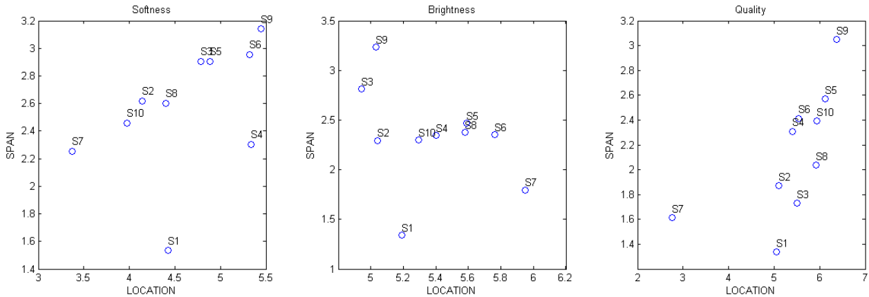
Figure 2. Plot of SPAN_j vs LOCATION_j for each subject and each descriptor.
