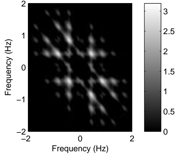
Bispectrum log-magnitude – Symmetric kernel
