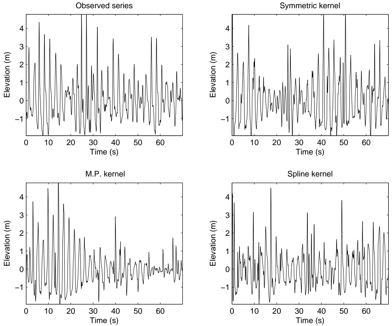
Figure 7: Example of trajectories of fitted processes.
