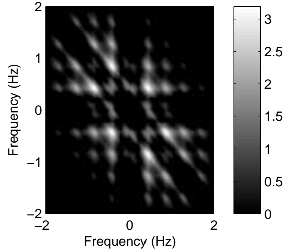
Bispectrum log-magnitude – Spline kernel
