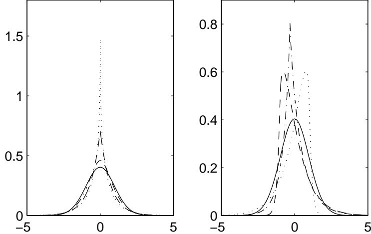
Figure 1: Densities of GAL distributions
