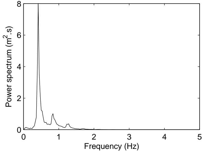
Figure 6: Power spectral density of observations.
