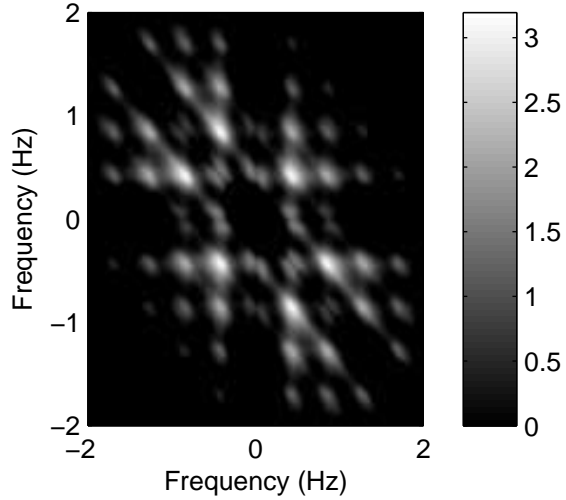
Bispectrum log-magnitude – M.P. kernel
