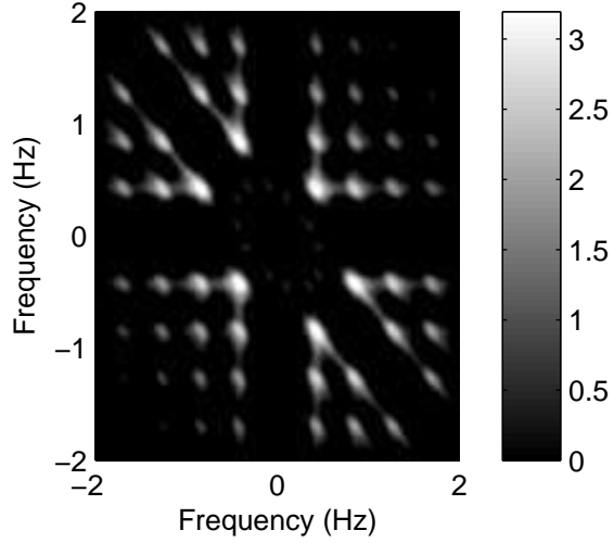
Bispectrum log-magnitude – Observations
