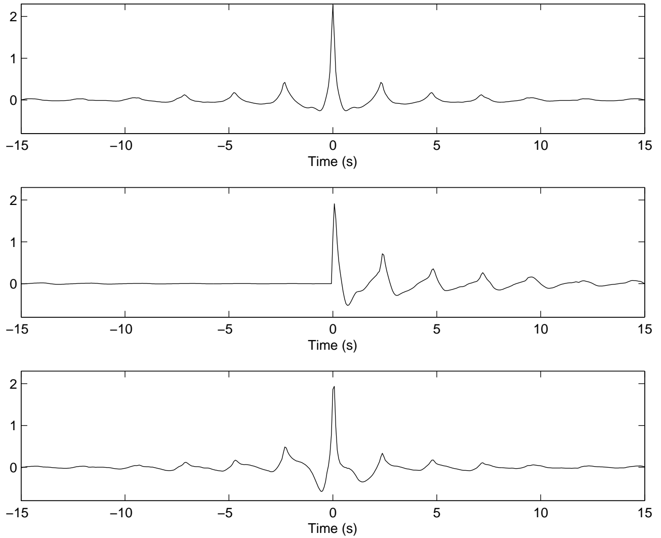
Figure 8: Estimated kernels. From top to bottom: symmetric model, minimum phase model, spline model.
