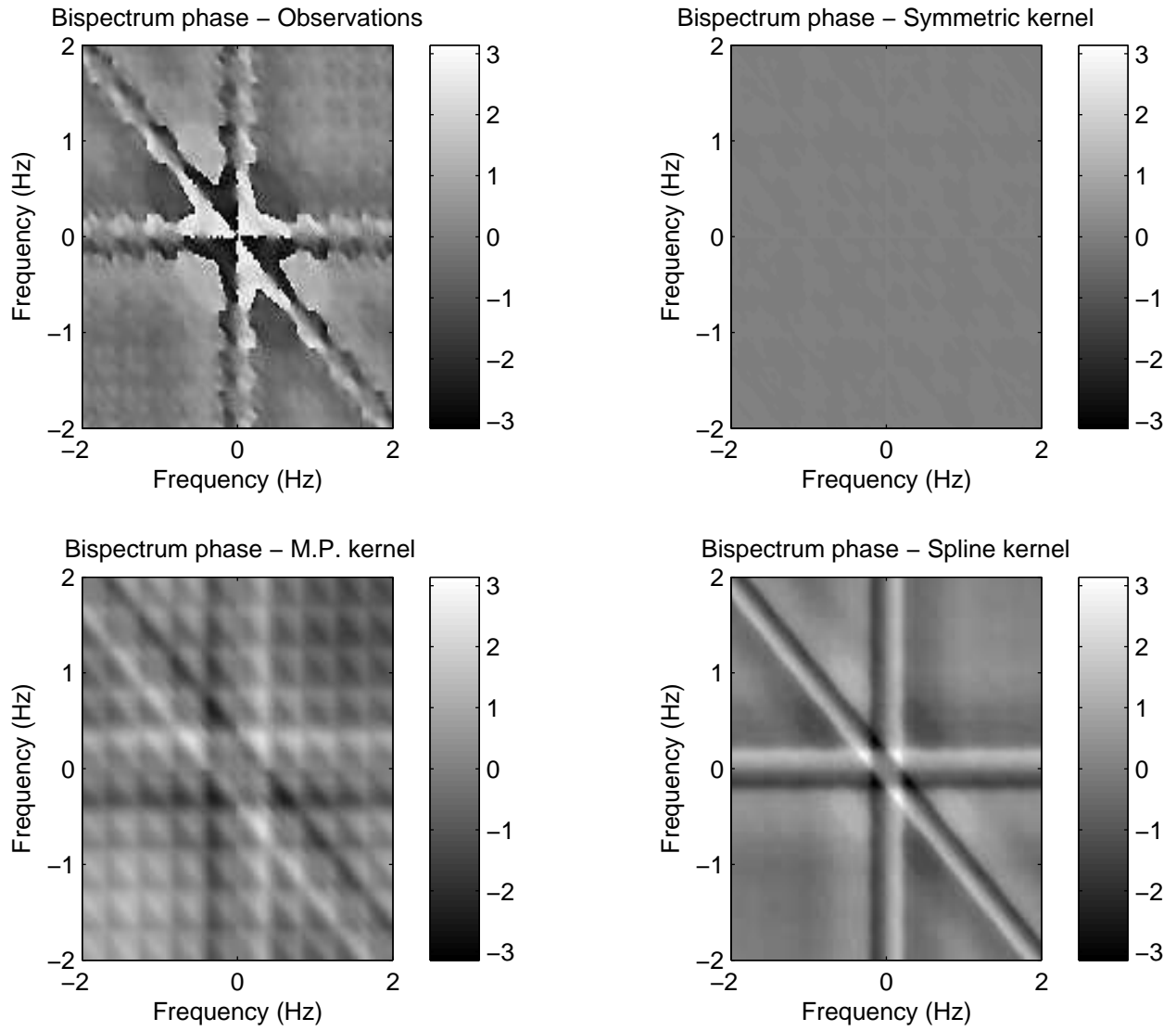
Figure 10: Angle of bispectra of observed process and fitted models.
