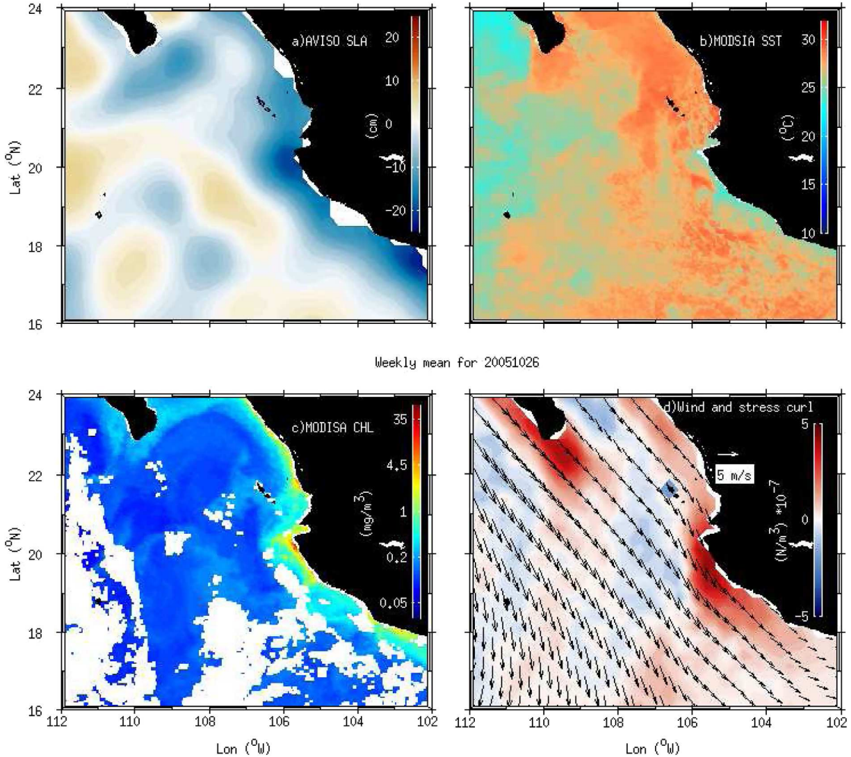
Figure 4. Surface conditions from remote sensing observations for 26 October 2005: (a) SLA (in cm), (b) SST (in ^{\circ}\text{C} ), (c) CHL (in \text{mg}/\text{m}^3 ), and (d) wind (in \text{m}/\text{s} black arrows) and wind stress curl (in 10^{-7} \text{ N}/\text{m}^3 , color shading).
