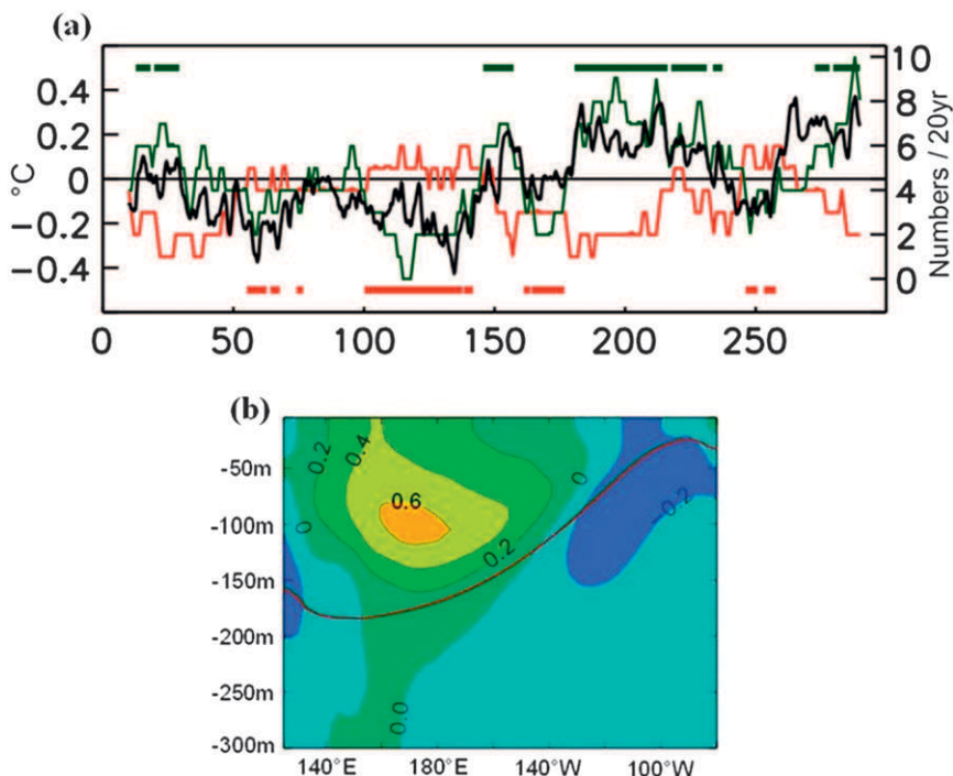
FIG. 6. (a) Decadal variability and decadal modulation of ENSO in the GFDL CM2.1 simulation, as a function of time from the beginning of the simulation ( x axis; yr). Green (red) thin line indicates 20-yr frequency of CP (EP) events, in numbers by 20-yr increments (right y axis). Black line indicates 20-yr running mean of SST averaged within Niño4m region ( ^{\circ}\text{C} ; left y axis). Green (red) horizontal thick lines in the top (bottom) indicate period intervals used to compute the warm (cold) mean state. Adapted from Kug et al. (2010) and Choi et al. (2011). (b) Temperature differences at the equator between the warm and cold mean states, as a function of longitude and depth. CI is 0.2^{\circ}\text{C} and the 20^{\circ}\text{C} isotherm depth is drawn for the cold mean state (red, almost identical for the warm mean state).
