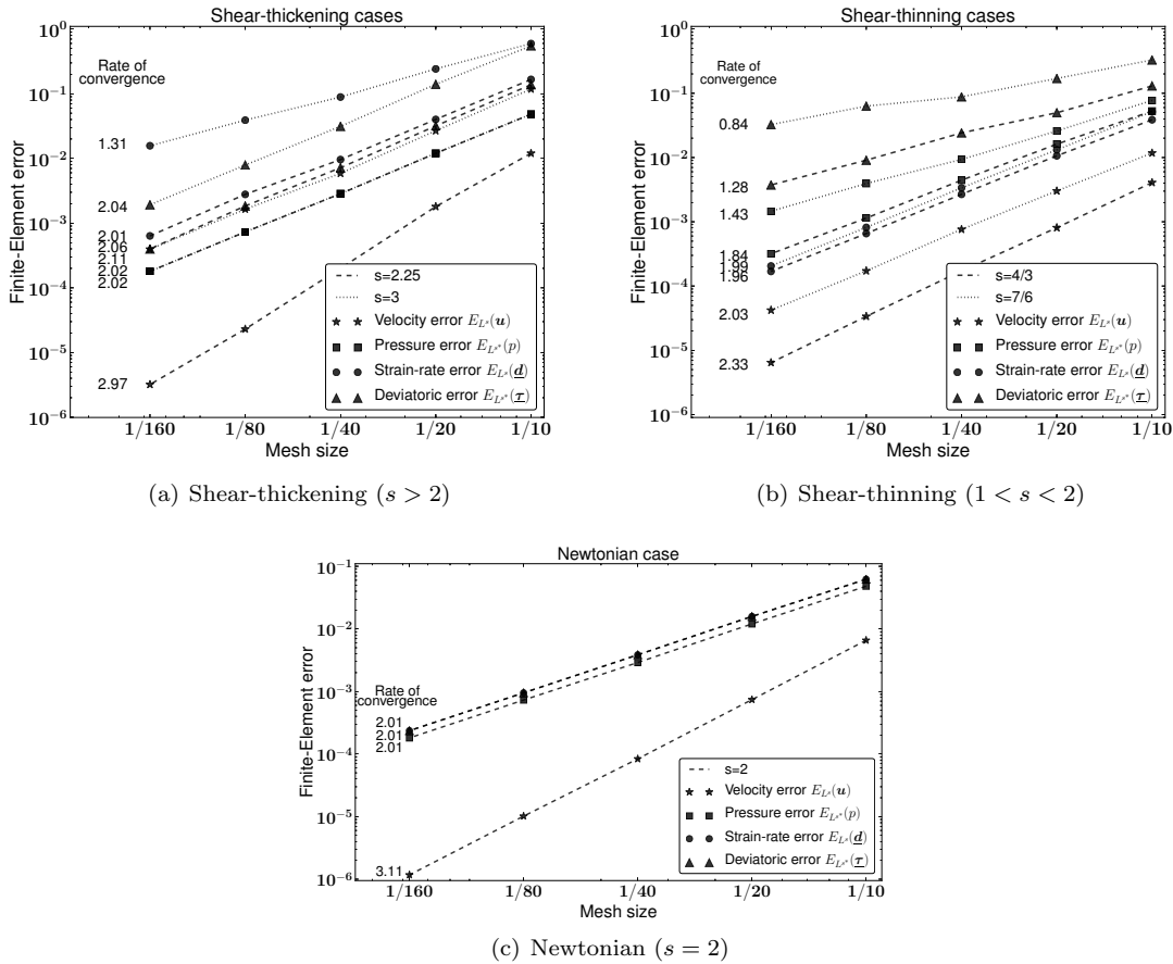
FIGURE 3. Convergence curves: variation with respect to the mesh-cell size h of the following finite element approximation errors (defined by (114)): E_{L^s}(\mathbf{u}) (Velocity error), E_{L^s}(\underline{\mathbf{d}}) (strain-rate error), E_{L^{s^*}}(p) (pressure error) and E_{L^{s^*}}(\underline{\boldsymbol{\tau}}) (deviatoric error). These errors have been computed using LA algorithm for various power-law exponent s ( s = 1.16, 1.33, 2.25 and 3 ; exact solution given by (112)). The rates of convergence indicate the average logarithmic slope. Pressure error is identical for s = 2.25 and s = 3 .
