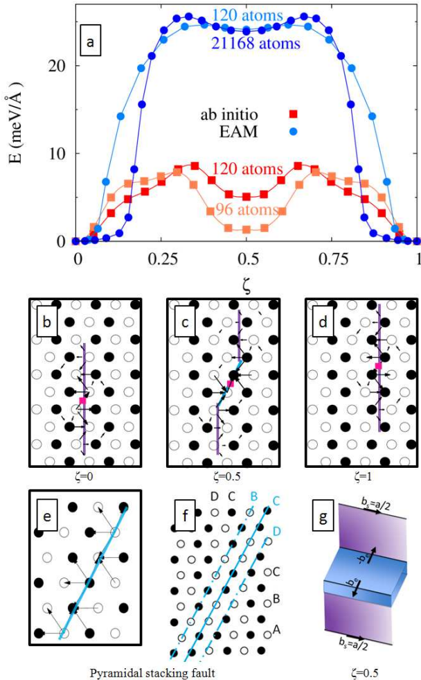
FIG. 2. Secondary slip in the pyramidal ( \bar{1}011 ) plane. (a) Energy barrier encountered by a screw dislocation dissociated in a prismatic plane when gliding in a pyramidal plane. Differential displacement maps show the dislocation in its (b) initial, (c) intermediate, and (d) final states. The arrow between two atomic columns is proportional to the relative displacement of the columns in the [1\bar{2}10] direction. Displacements smaller than 0.08b are not shown. The pink squares indicate the dislocation center. The pyramidal stacking fault is shown through its differential displacement map with respect to a perfect crystal in (e) and through its stacking sequence in (f), so as to display the two mirror planes ( B and D ) associated with the twin structure. The intermediate dislocation configuration is sketched in (g). The prismatic and pyramidal faults are shown in blue and purple, respectively.
