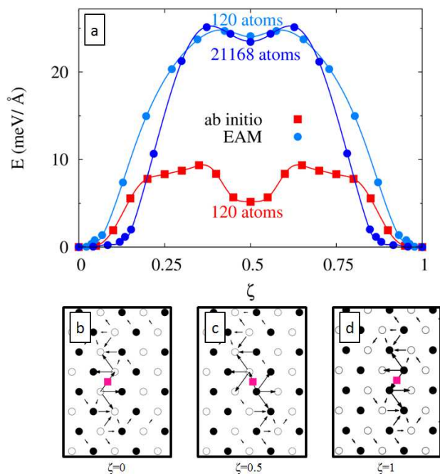
FIG. 3. Secondary slip in the basal (0001) plane. (a) Energy barrier encountered by a screw dislocation when gliding in a basal plane. The differential displacement maps show the dislocation (b) initial, (c) intermediate, and (d) final configurations.
