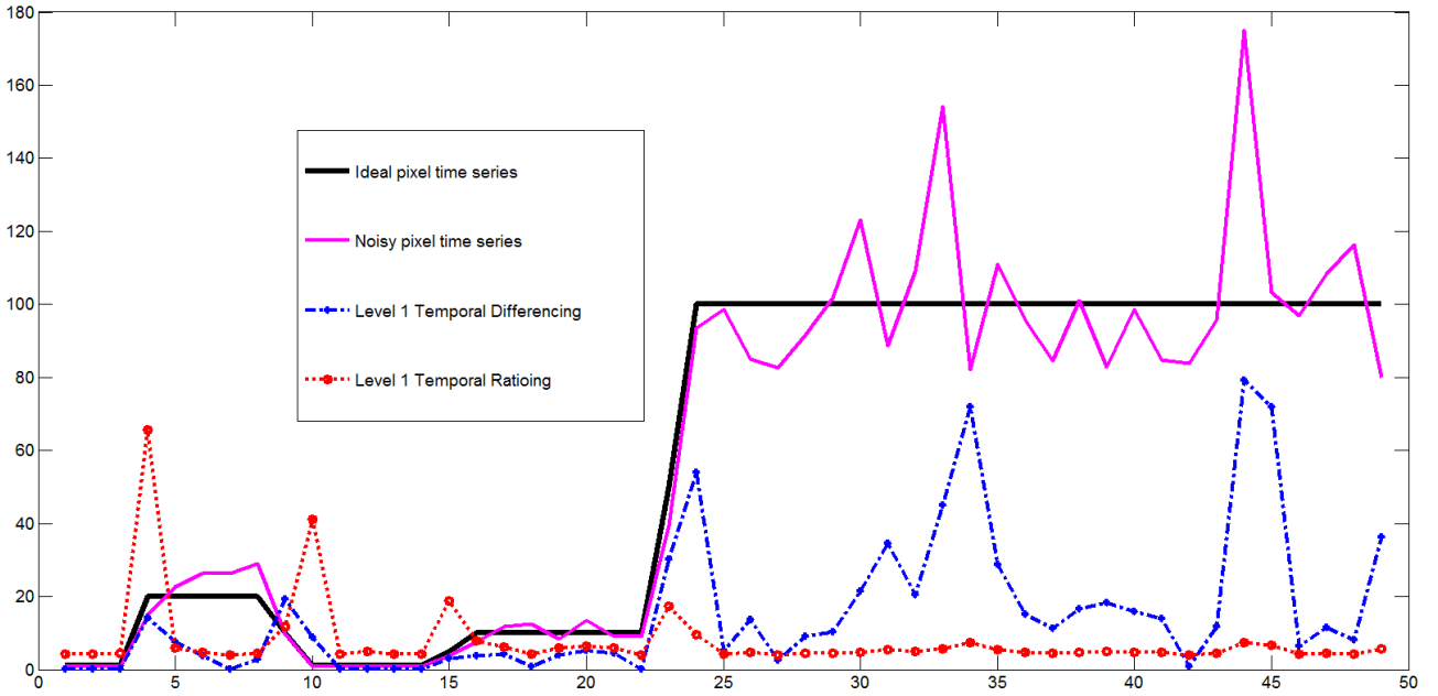
Fig. 1. Pixel time series with 4 change dates, its noisy speckled version, as well as absolute change information from arithmetic differencing (corresponds to Haar level-1 ADWT details) and ratioing (geometric differencing, corresponds to Haar level-1 non sub-sampled GDWT details). The ratio-data have been re-scaled logarithmically so as to make comparison on a single display possible.
