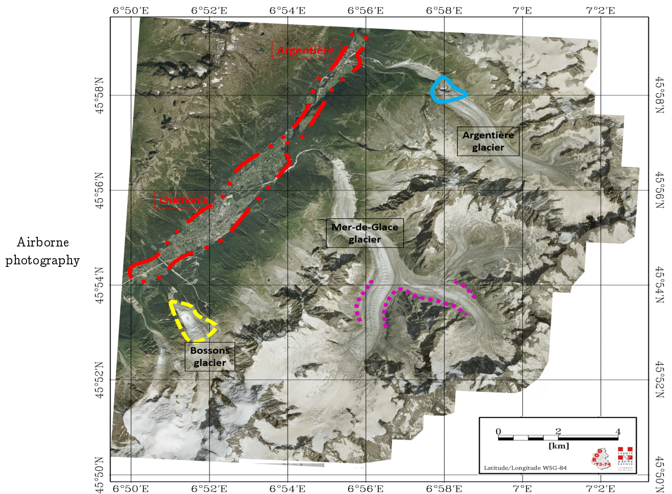
Fig. 6. Top: 1 sample geometric change-image of PolSAR time series \mathcal{P} described in Figure 5. Bottom: airborne photography [©RGD 73-74] showing Chamounix urban valley (red dash-dotted), glaciers ( Argentière , Mer de Glace , Bossons ) and localization of significant changes.
